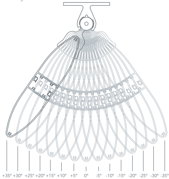
Vertical blade angle settings: 15 different angles ranging from +35 to -35 degrees with 5 degree increments.
